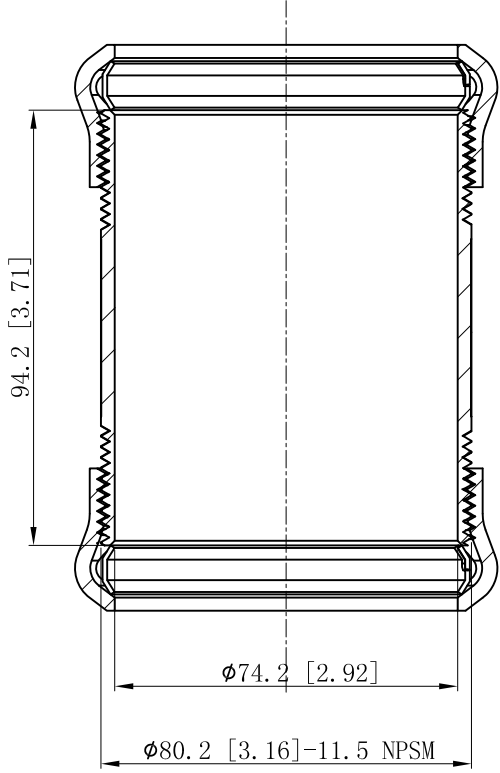
CUTAWAY VIEW A-A
