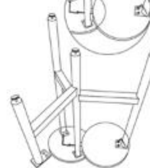
Fix Mid Shelf with mid leg use small Allen screws in bottom side and large Allen screw in side leg
