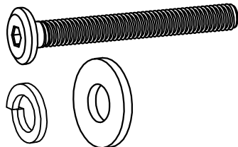
ALLEN KEY BOLT: M8 X 60mm - QTY 8 LOCK WASHER: Ø12 / Ø8 X 1.5mm - QTY 8 WASHER: Ø19 / Ø8 X 1mm - QTY 8 QTY 8 SETS
