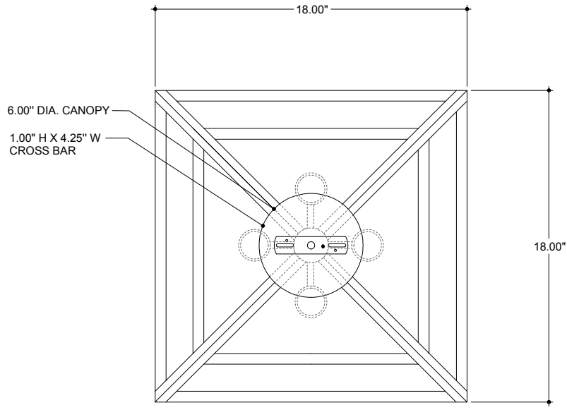
CANOPY DETAIL
