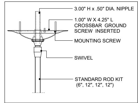
CANOPY DETAIL
