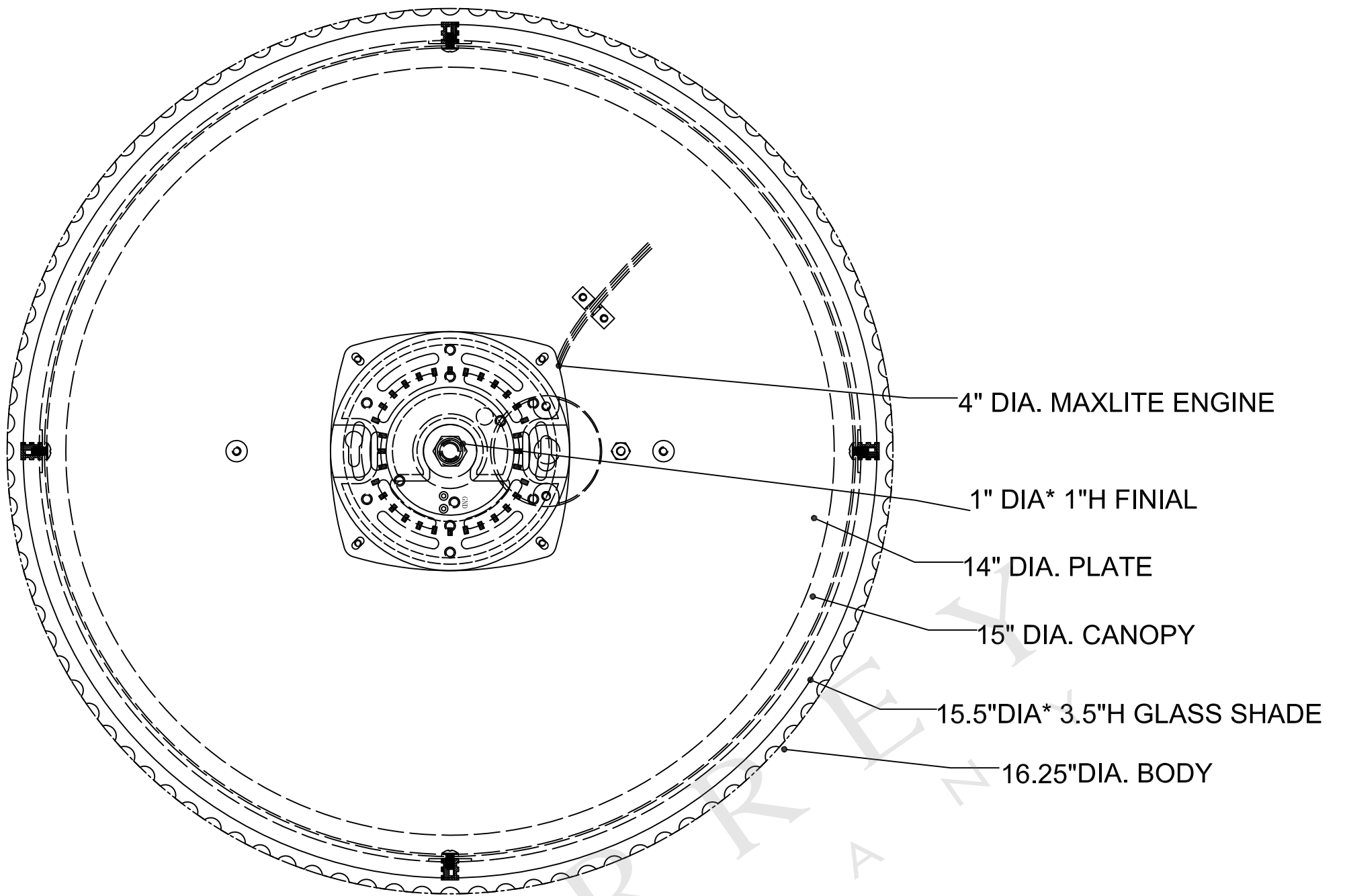
TOP VIEW
