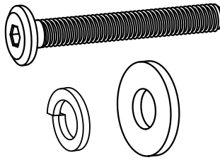
ALLEN KEY BOLT: M8 X 50mm - QTY 8 LOCK WASHER: \varnothing 12 / \varnothing 8 \times 1.5 mm - QTY 8 WASHER: \varnothing 19 / \varnothing 8 \times 1 mm - QTY 8 QTY 8 SETS
