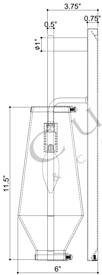
SIDE VIEW
