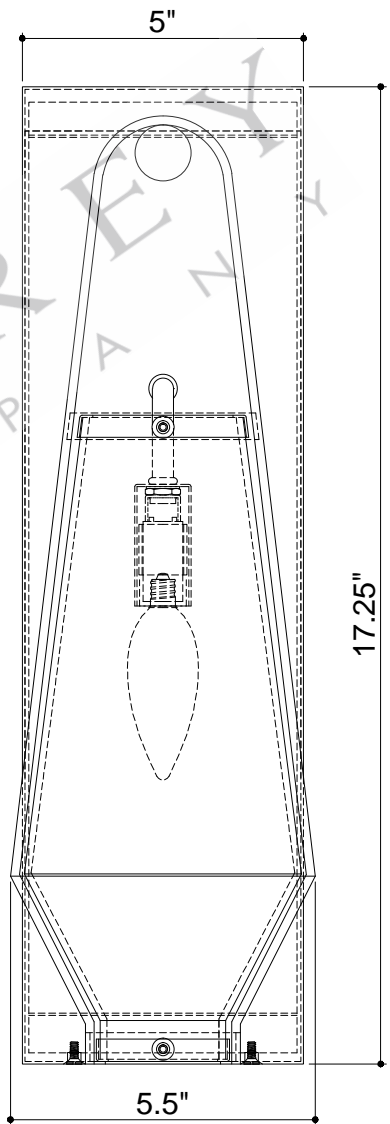
FRONT VIEW
