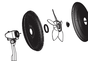
1. Assemble Fan Head.
