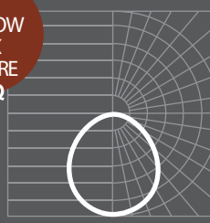
Diffuse-Lambertian
