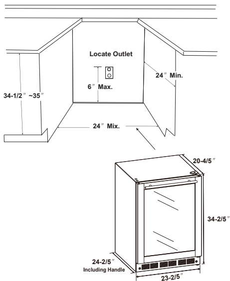
Figure A – The cutout depth must be 24"
