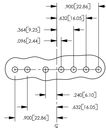
CAVITY LAYOUT
