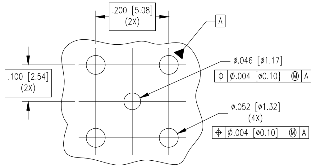
RECOMMENDED HOLE PATTERN
