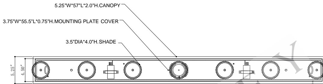
TOP VIEW
