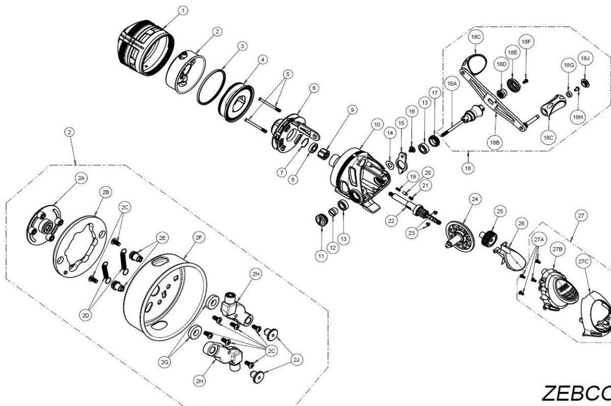
Zebco Bullet Spincast Reel Part List
