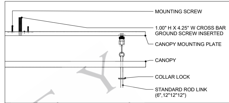
CANOPY DETAIL
