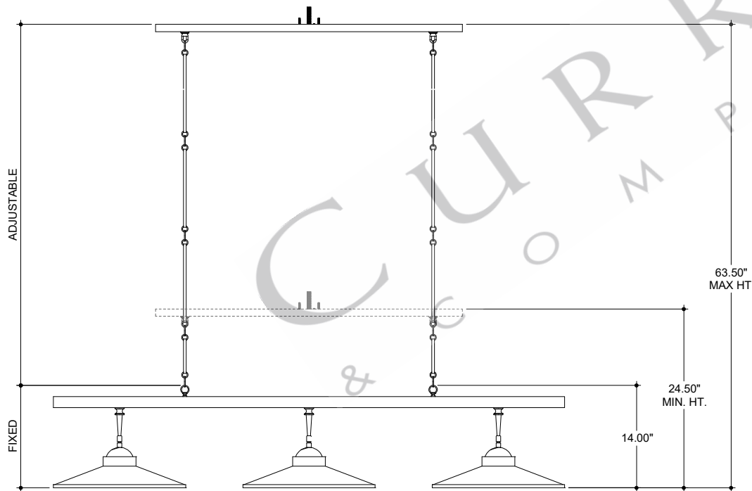
FRONT VIEW
