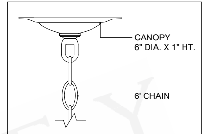
CANOPY DETAIL
