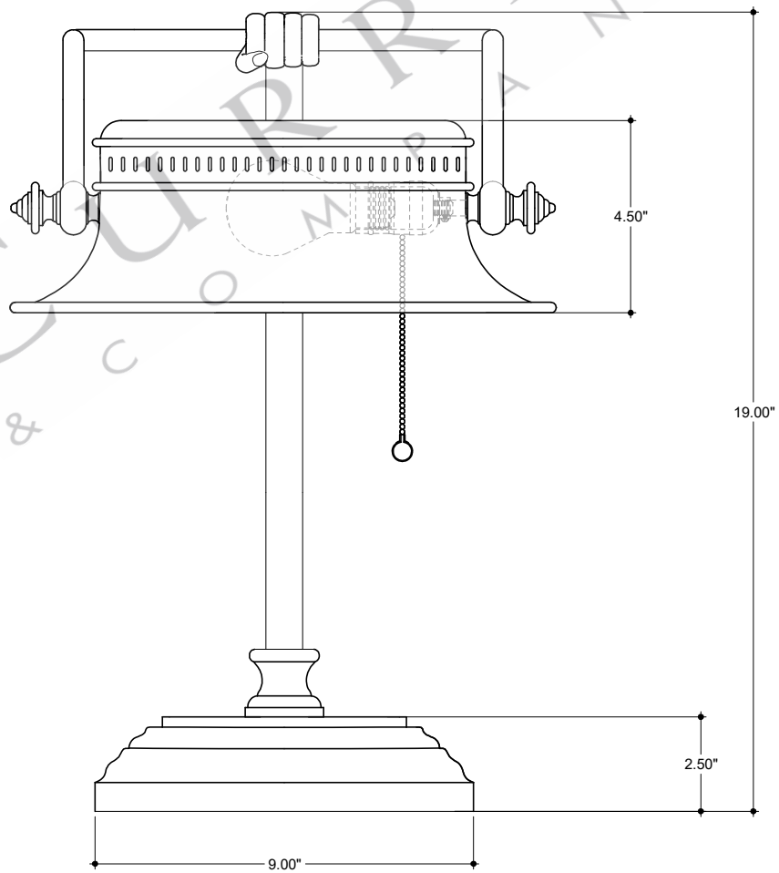
FRONT VIEW
