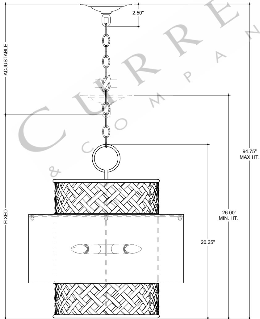
FRONT VIEW
