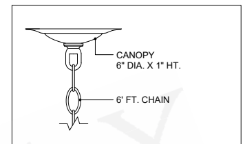
CANOPY DETAIL
