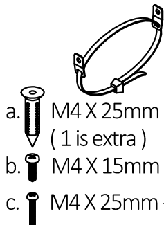
FURNITURE TIP OVER RESTRAINT QTY 1 SET
