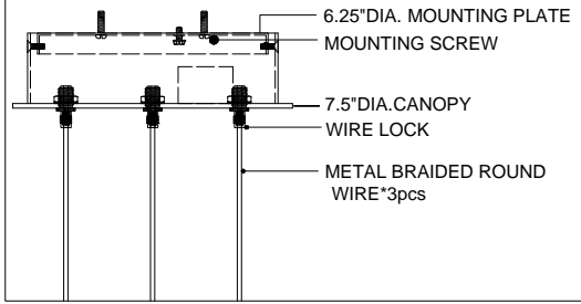
CANOPY DETAIL
