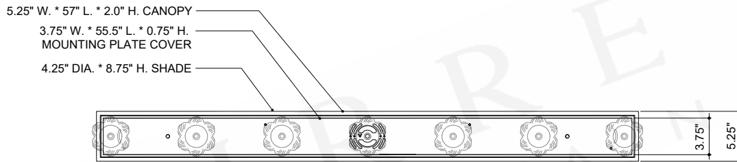
TOP VIEW
