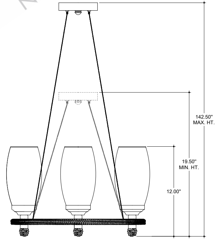
SIDE VIEW
