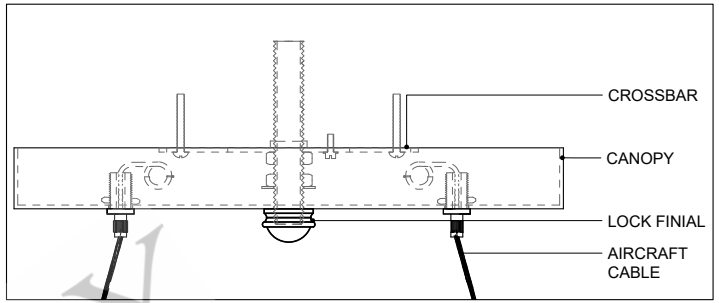
CANOPY DETAIL
