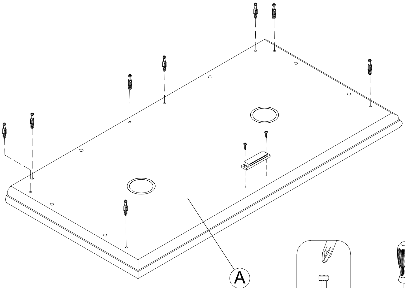
KD Bolt
