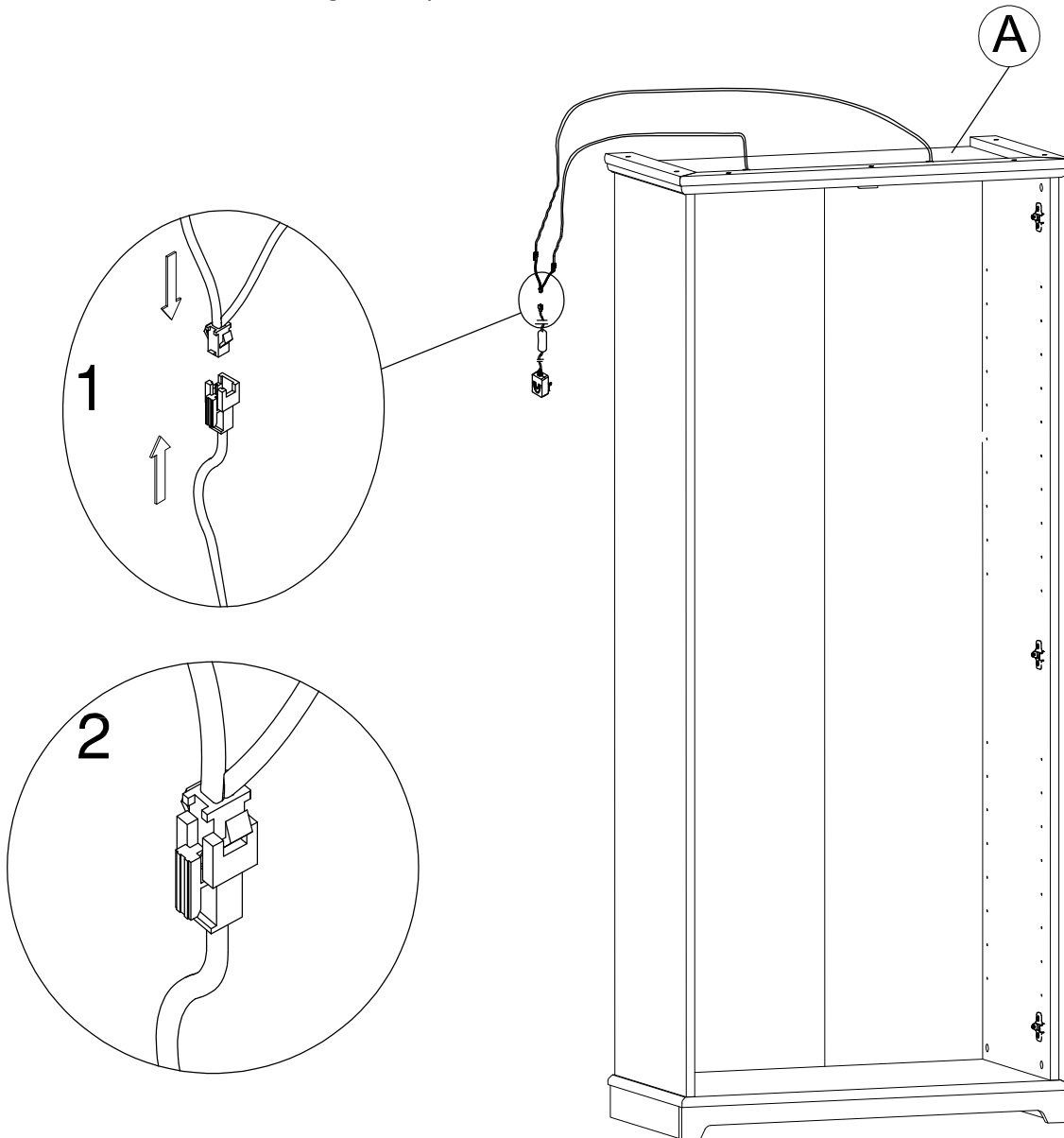
Light Adaptor
