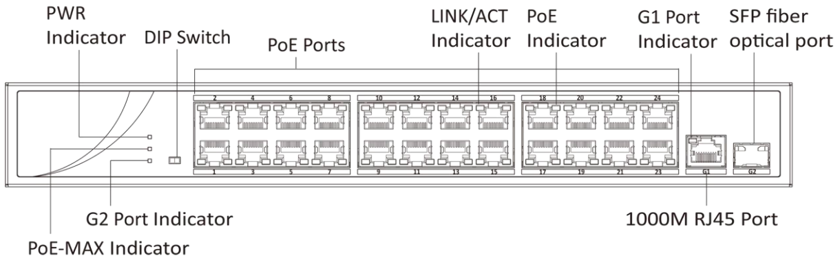
Figure 1-2 DS-3E0326P-E/M(B) Front Panel
