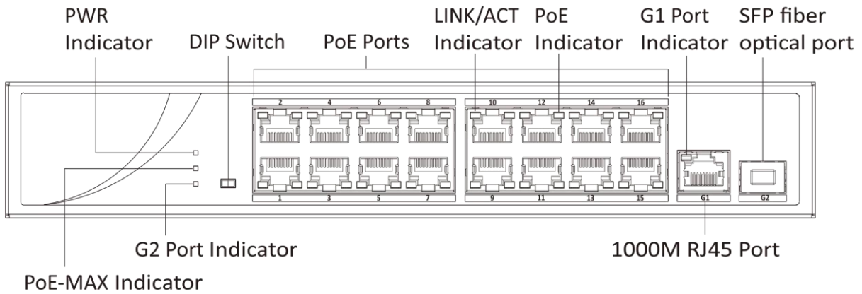
Figure 1-1 DS-3E0318P-E/M(B) Front Panel
