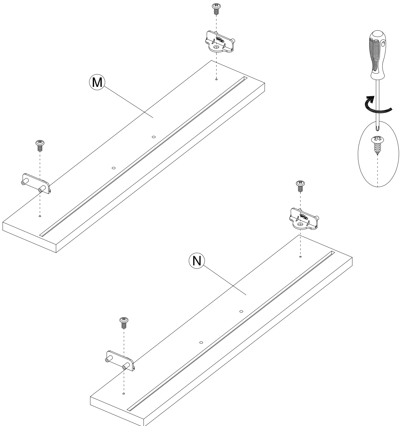
Drawer Bracket
