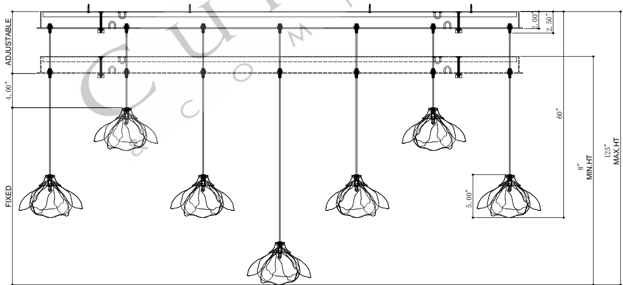
FRONT VIEW
