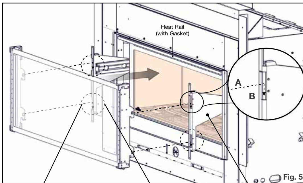
TGG slider bracket
