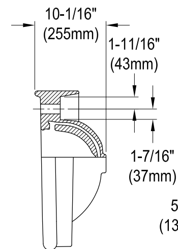
Sink Section A-A
