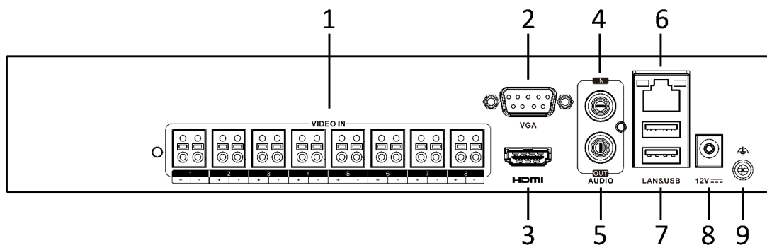
Figure 1-23 Rear Panel of DS-7208HGHI-F1/NB
