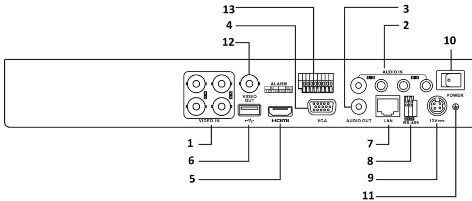
Figure 1-16 Rear Panel of DS-7200HUHI and 7600HUHI-F/N
