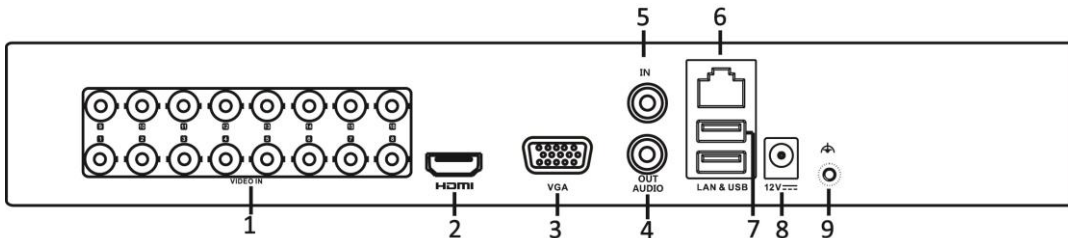
Figure 1-13 Rear Panel of DS-7200HGHI-E
