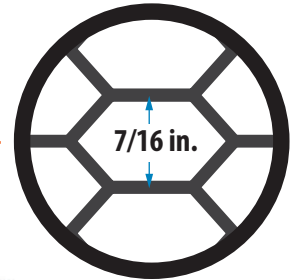
Mesh Detail
