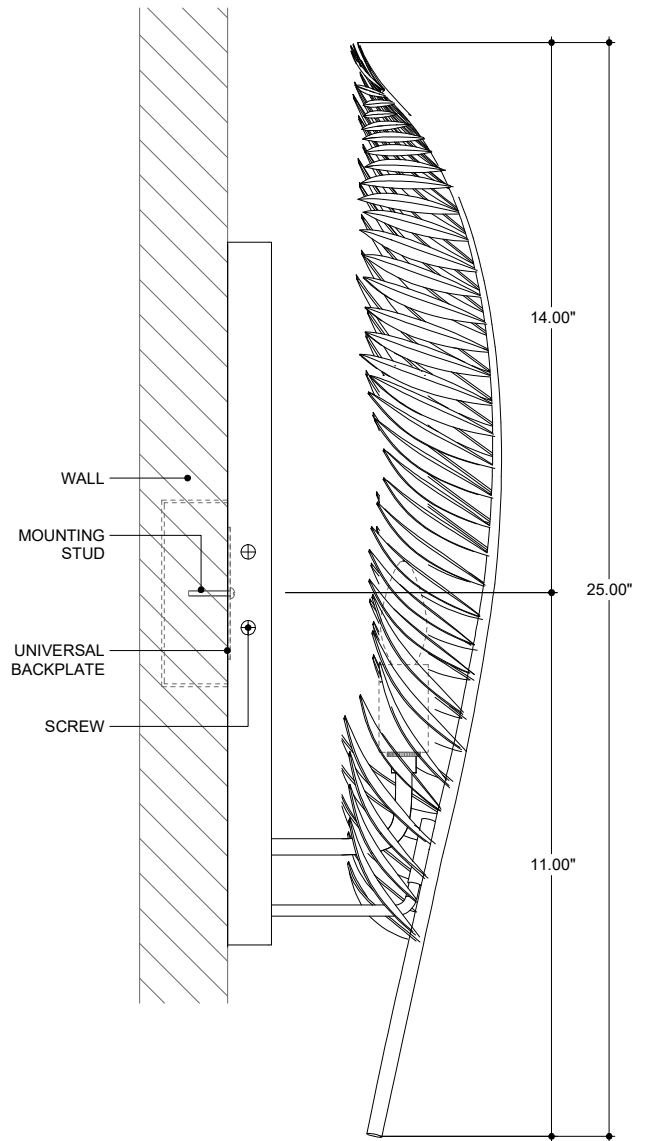
SIDE VIEW
