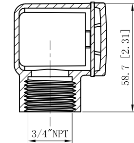
CUTAWAY VIEW B-B
