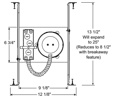
4 1/2" CEILING CUTOUT
