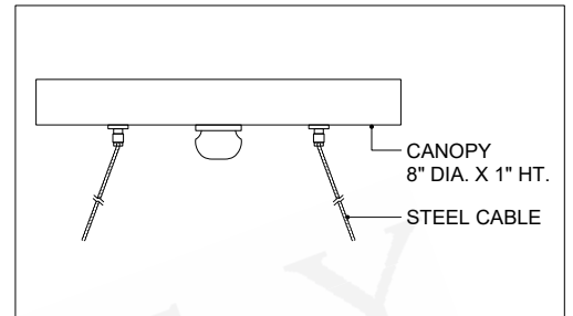
CANOPY DETAIL
