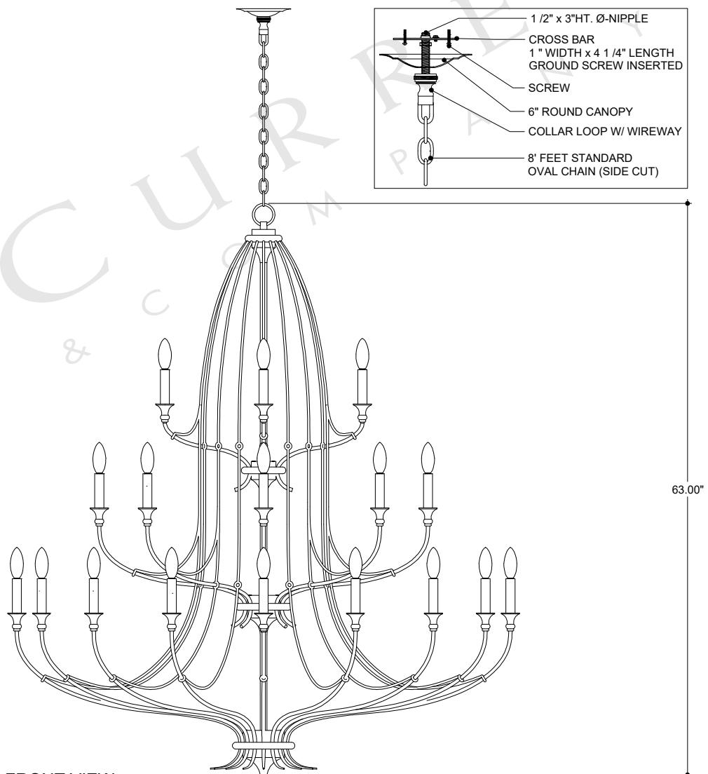
FRONT VIEW
