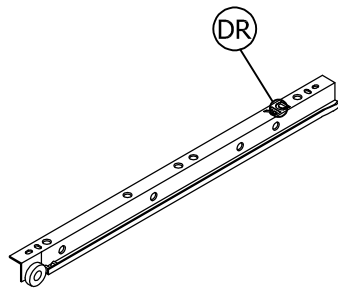
14" Slide Runner(356mm)
