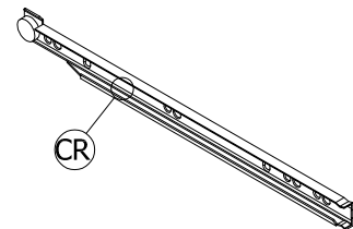
14" Slide Mount(356mm)
