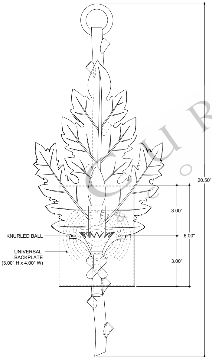
FRONT VIEW
