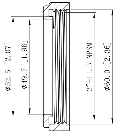
CUTAWAY VIEW A-A
