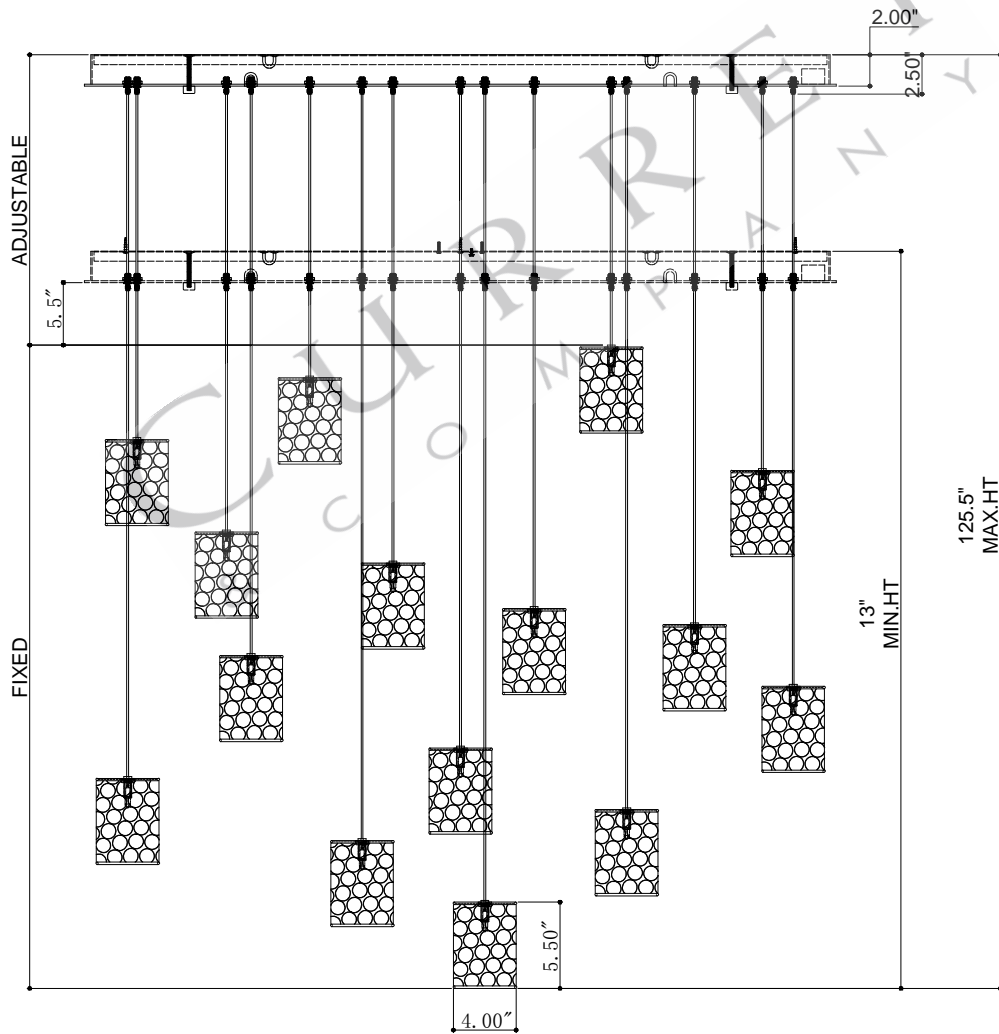
FRONT VIEW
