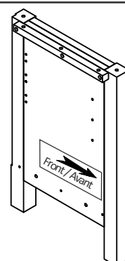
RIGHT SIDE QTY 1
