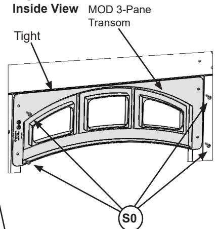
Fig. 12.4 Inside View
