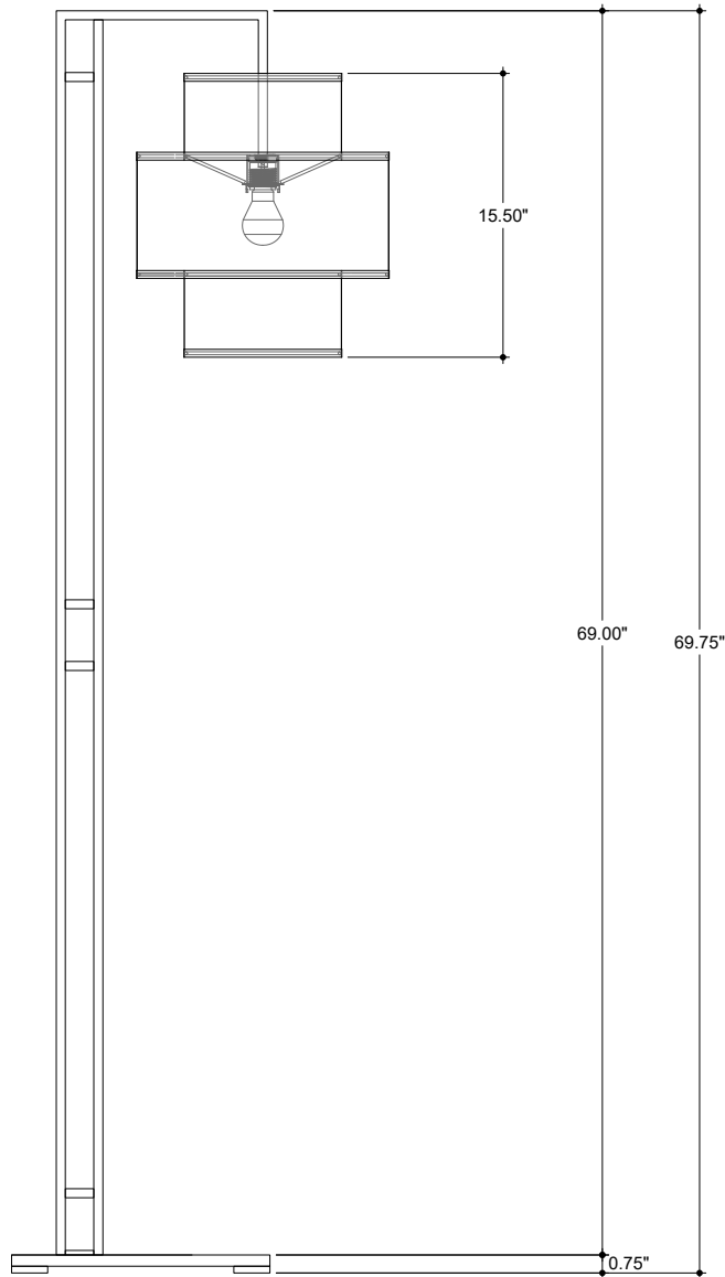
FRONT VIEW
