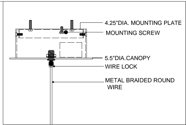
CANOPY DETAIL
