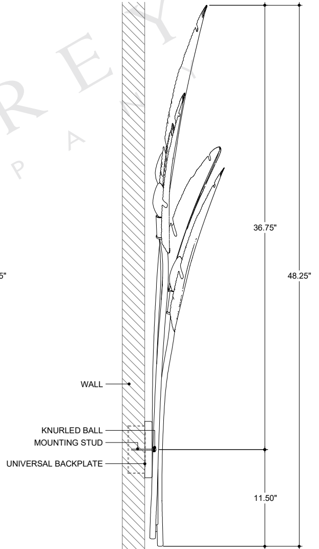
SIDE VIEW
