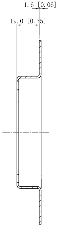
CUTAWAY VIEW A-A
