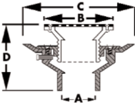
DRAIN DIMENSIONS
