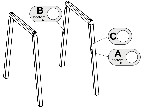
1x left leg (with A B C stickers)
