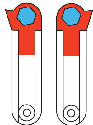
VIEWS OF BOTTOM HINGE SEEN FROM BELOW BEFORE AND AFTER REVERSING THE STOP
